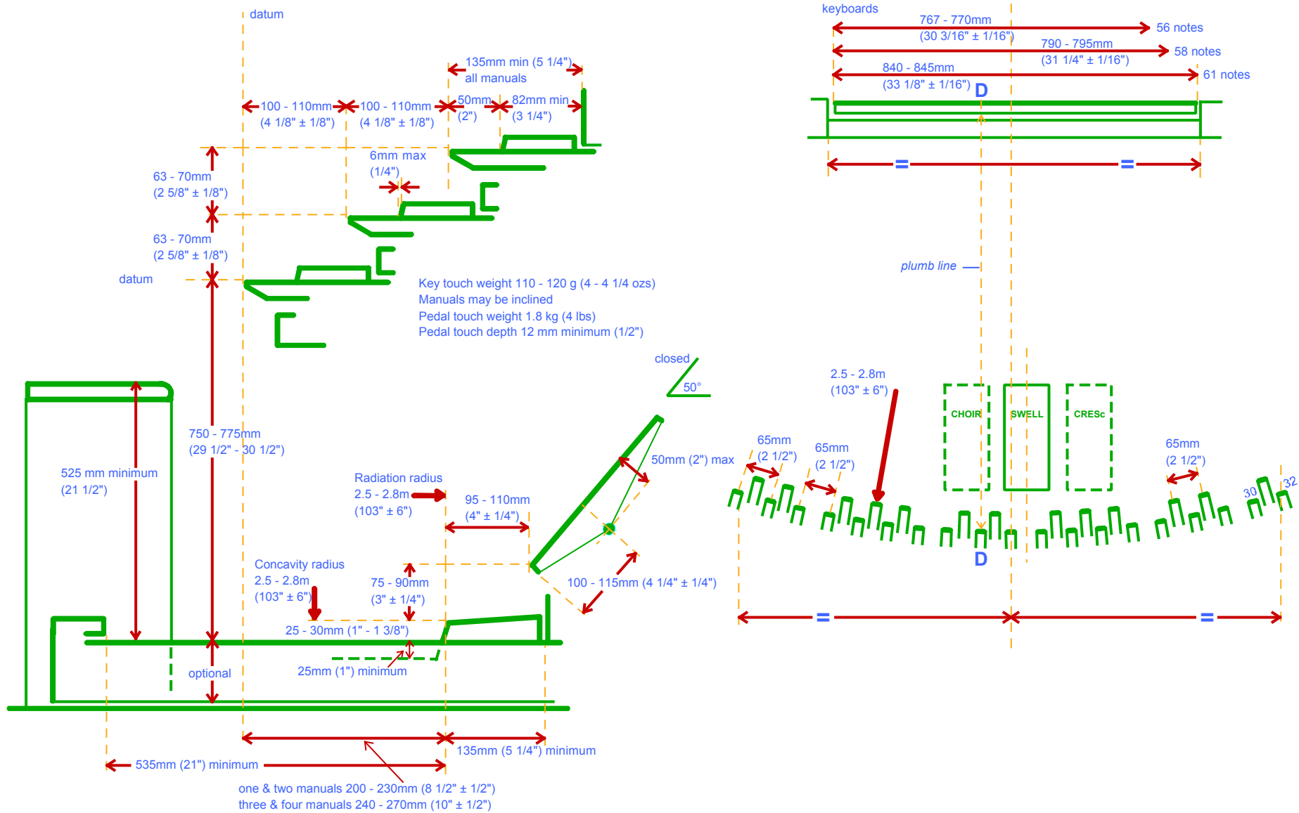
BRITISH ORGAN CONSOLE DIMENSIONS - RECOMMENDED STANDARD - 1967
